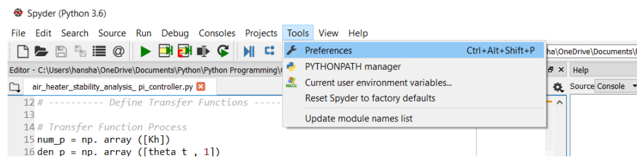
Figure 17.2: Python Tools-Preferences
