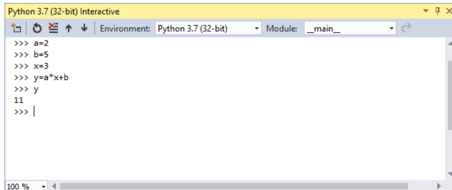
Figure 19.4: Python Interactive
