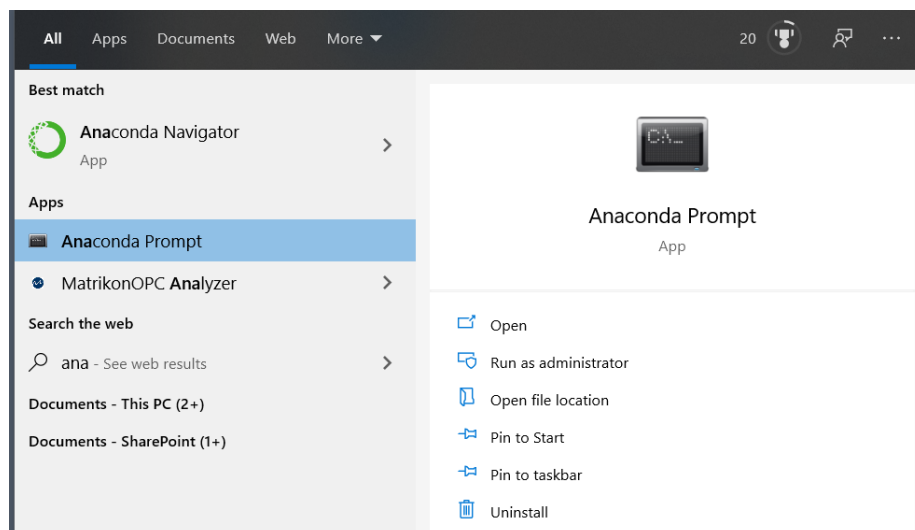
Figure 14.2: Anaconda Navigator
